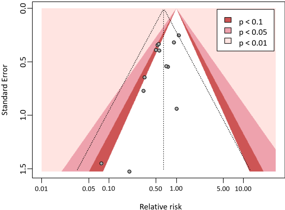
Comparison-adjusted funnel plot (SSI)
