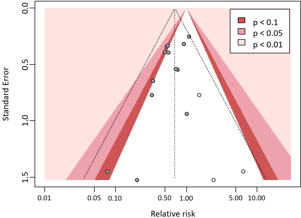
Comparison-adjusted funnel Plot (Trim & Fill Method)
